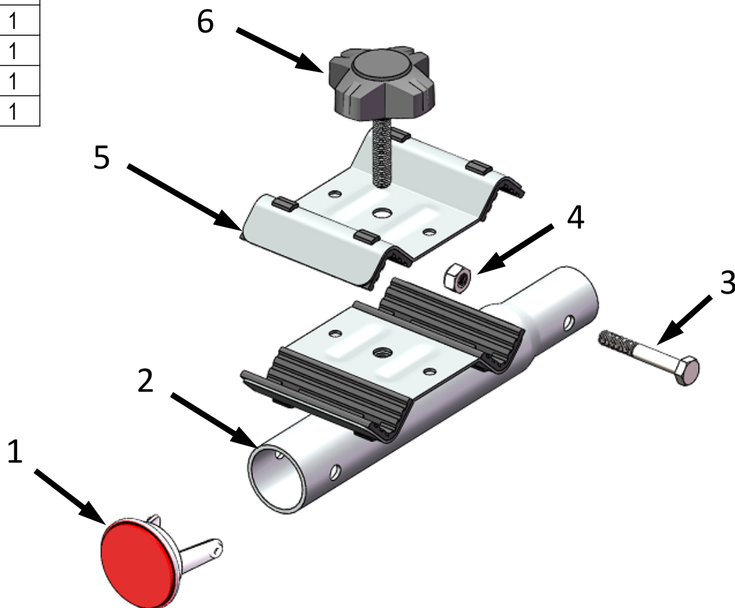
Parts Diagram
